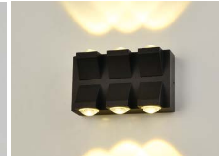
GMD-F689A-3 Lamp:LED 6 × 1W Size:D140 × W50 × H95
