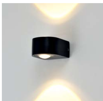
GMD-F819Y-2 Lamp:LED 2 × 3W Size:D70 × W85 × H50
