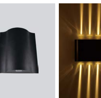
GMD-F688-2 Lamp:LED 2 × 3W Size:D165 × W65 × H210
