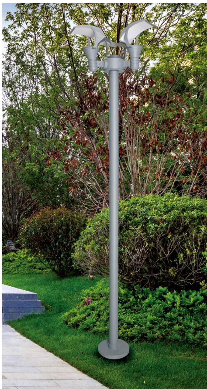
GMD-2088S-3 MR16×3 LED:(5×1W)×3 Size:Φ115×H2000mm
