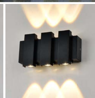
GMD-F815B-3 Lamp:LED 6 × 1W Size:D170 × W45 × H90
