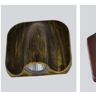
GMD-F695-1 Lamp:LED 3W Size:D145 × W65 × H150
