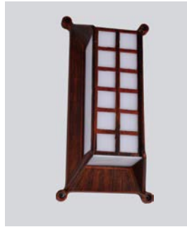
GMD-F59 Lamp:E27/LED 1 × 10W Size:D160 × W110 × H330
