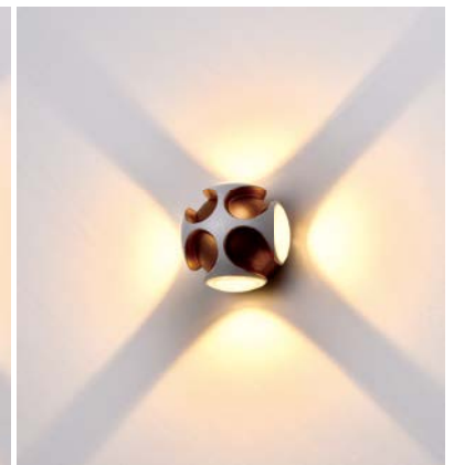
GMD-828D-S Lamp:LED 4 × 3W Size:Φ 90 × H85
