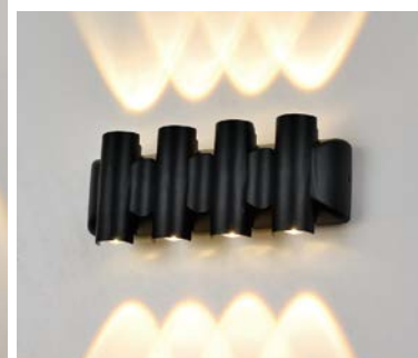
GMD-F815A-4 Lamp:LED 8 × 1W Size:D220 × W45 × H90
