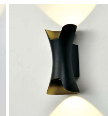
GMD-F857Y Lamp:LED 2 × 5W Size:D100 × W95 × H200
