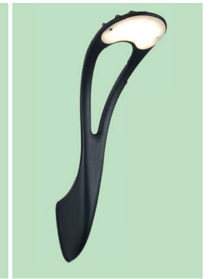
GMD-F823 Lamp:LED 10W Size:D130 x W290 x H420
