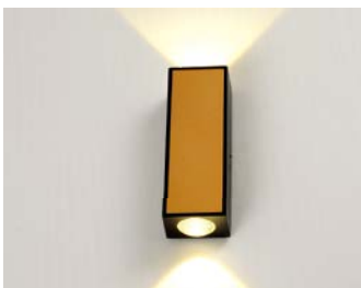
GMD-F496/S-2 Lamp:LED 2 × 3W Size:D50 × W40 × H145
