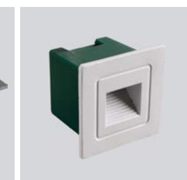
GMD-D690S Lamp:LED 1 × 1W Size:D55 × W55 × H45
