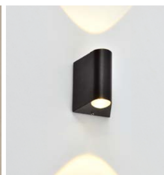
GMD-F560 Lamp:LED 2 × 3W Size:D60 × W60 × H95
