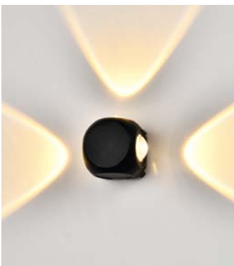
GMD-828F/S-3 Lamp:LED 3 × 1W 3030 Size:Φ 65
