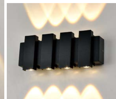
GMD-F815B-4 Lamp:LED 8 × 1W Size:D220 × W45 × H90
