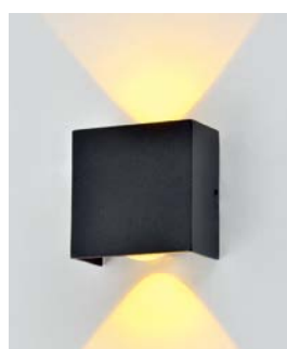
GMD-F813B-1 Lamp:LED 2 × 3W Size:D80 × W50 × H60
