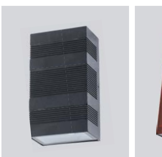
GMD-F683带条纹 Lamp:LED 2 × 3W Size:D95 × W55 × H160
