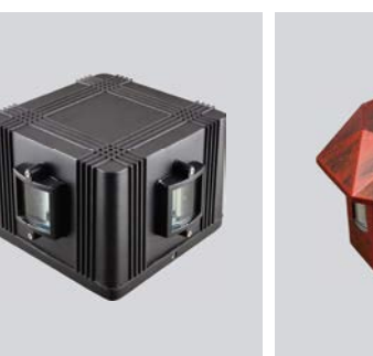
GMD-2007-4 Lamp:E14/LED 4 × 3W Size:D195 × W115 × H195
