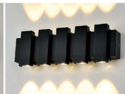
GMD-F815B-5 Lamp:LED 10 × 1W Size:D280 × W45 × H90
